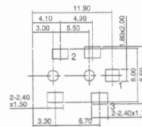
PIN HOLE LAYOUT (BOTTOM VIEW)
