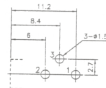
PIN HOLE LAYOUT (BOTTOM VIEW)
