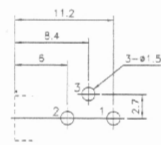
PIN HOLE LAYOUT (BOTTOM VIEW)
