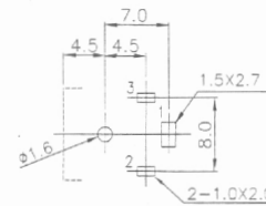
PIN HOLE LAYOUT (BOTTOM VIEW)
