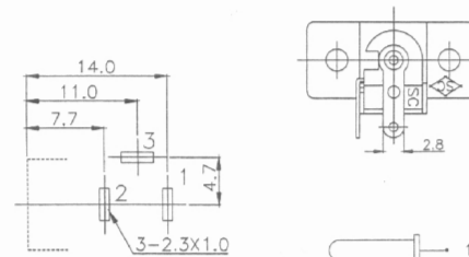
PIN HOLE LAYOUT (BOTTOM VIEW)
