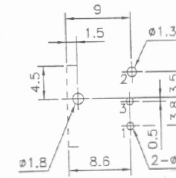
PIN HOLE LAYOUT (BOTTOM VIEW)
