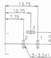
PIN HOLE LAYOUT (BOTTOM VIEW)
