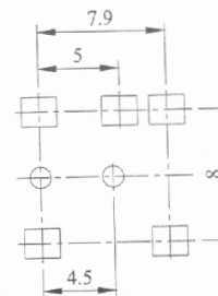
PIN HOLE LAYOUT (BOTTOM VIEW)
