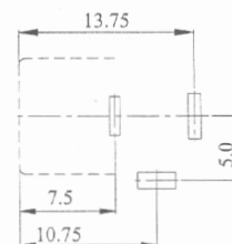
PIN HOLE LAYOUT (BOTTOM VIEW)
