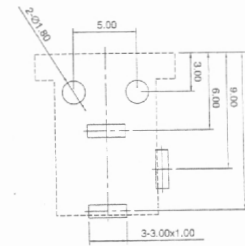
PIN HOLE LAYOUT (BOTTOM VIEW)
