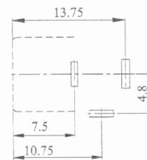
PIN HOLE LAYOUT (BOTTOM VIEW)
